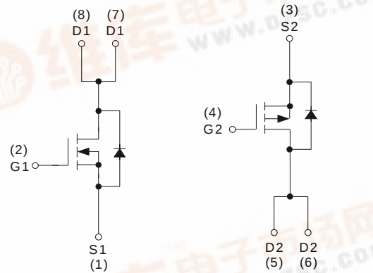
N-Channel MOSFET
