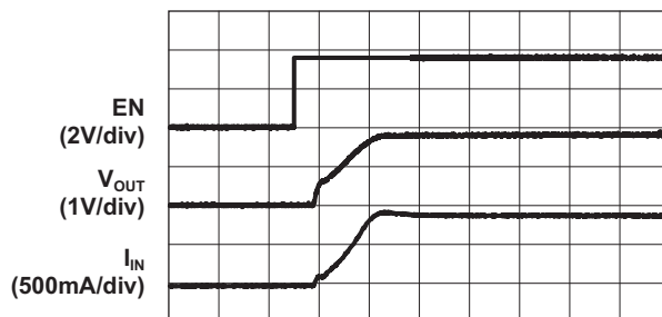
Enable Soft Start ( V_{IN} = 3.6V ; V_{OUT} = 1.8V ; I_{OUT} = 1.5A )
