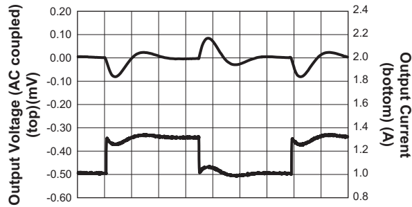
Load Transient Response ( V_{OUT} = 1.8V )
