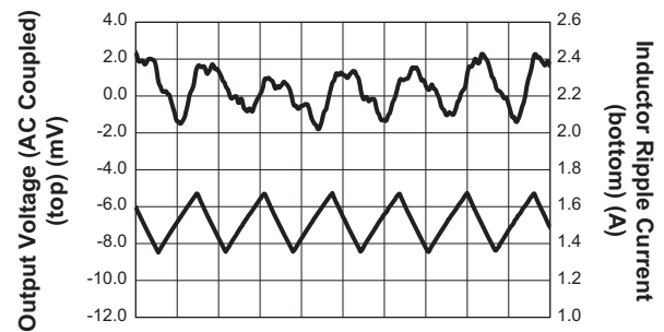
Heavy Load Switching Waveform ( V_{IN} = 3.6V ; V_{OUT} = 1.8V ; I_{OUT} = 1.5A )
