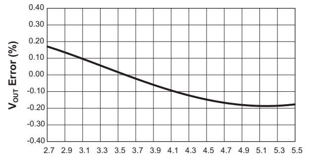
Line Regulation ( V_{OUT} = 1.8V ; I_{OUT} = 1A )
