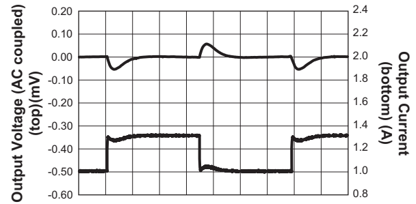
Load Transient Response ( V_{OUT} = 1.8V ; C_{FF} = 100pF )
