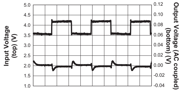
Line Transient Response ( V_{OUT} = 1.8V ; I_{OUT} = 1.5A ; C_{FF} = 100pF )
