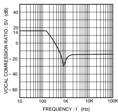
Fig. 5 SV vs. frequency characteristic
