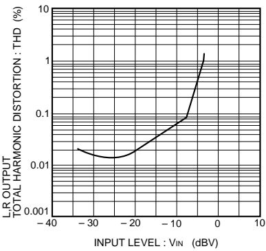
Fig. 6 THD vs. V_{IN} characteristics
