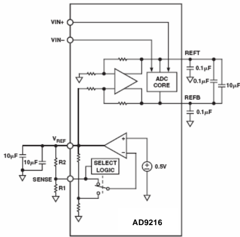
Figure 9. Programmable Reference Configuration
