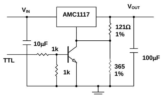
5V Regulator with Shutdown
