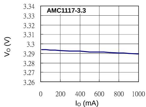
Load Regulation
