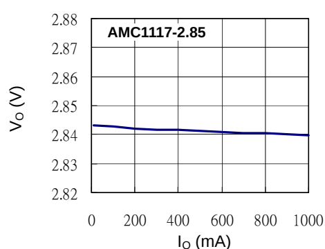
Load Regulation
