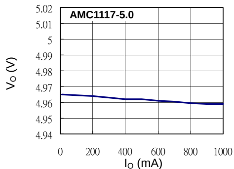
Load Regulation
