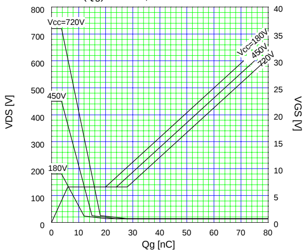
Typical gate charge characteristic
