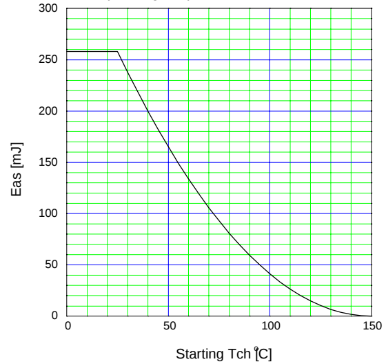
Avalanche energy derating
