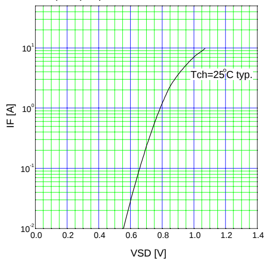
Forward characteristic of reverse of diode
