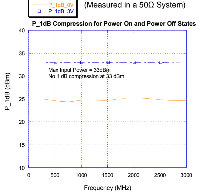
Figure 10. P_1dB Compression (Measured in a 50Ω System)
