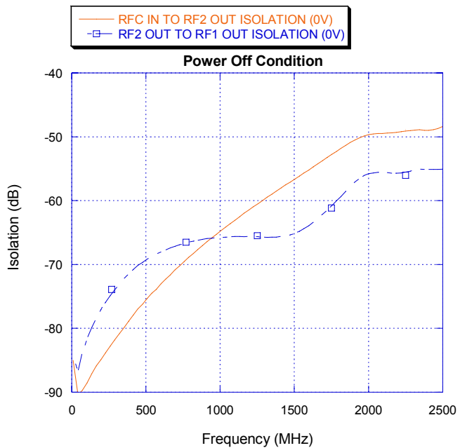
Figure 8. Isolation - Power Off
