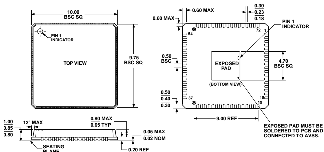
Figure 44. 72-Lead Lead Frame Chip Scale Package [LFCSP_VQ] 10 mm × 10 mm, Very Thin Quad (CP-72-1) Dimensions shown in millimeters
