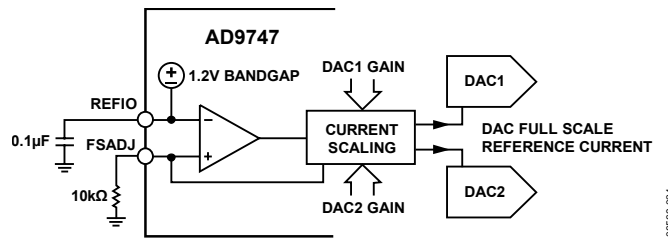
Figure 33. Reference Circuitry
