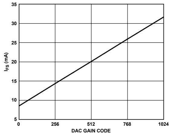
Figure 34. I_{FS} vs. DAC Gain Code
