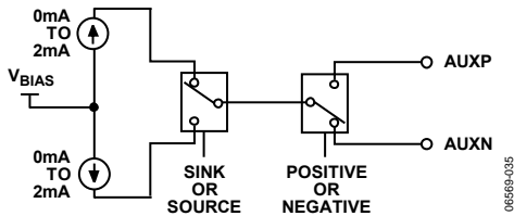
Figure 37. Auxiliary DAC Functional Diagram
