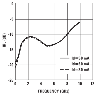
Figure 16. Input Return Loss vs. I d and Frequency.
