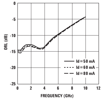
Figure 17. Output Return Loss vs. I d and Frequency.
