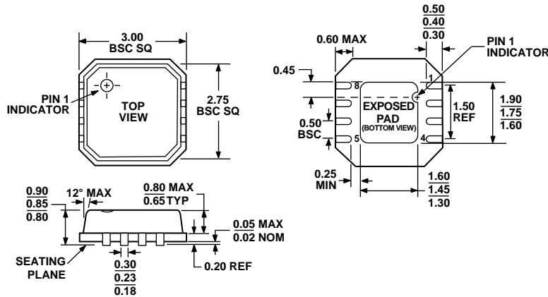
Figure 71. 8-Lead Lead Frame Chip Scale Package (LFCSPP) 3 mm x 3 mm Body (CP-8-2)—Dimensions shown in millimeters
