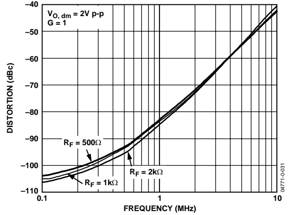
Figure 30. Third Harmonic Distortion at Various R_F
