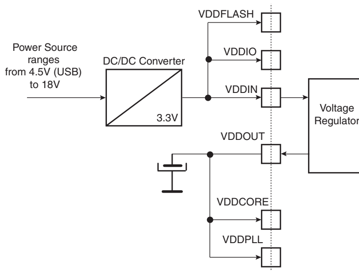
Figure 6-1. 3.3V System Single Power Supply Schematic
