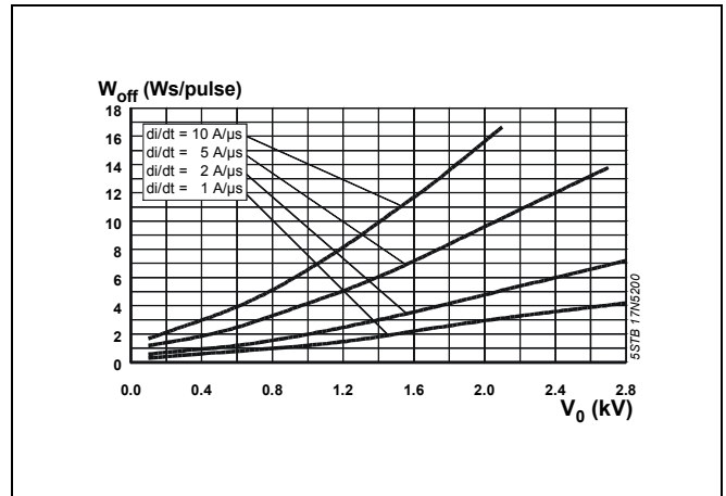
Fig. 18 W_{off} = f(V_0, di/dt) , T_j = 125\text{ }^\circ\text{C} . Rectangular waves.
