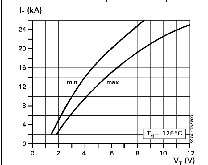
Fig. 2 On-state characteristics.
