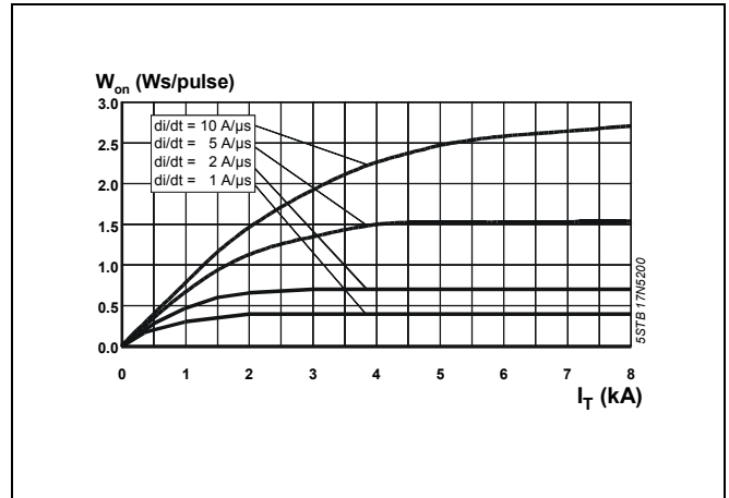
Fig. 16 W_{on} = f(I_T, di/dt) , T_j = 125\text{ }^\circ\text{C} . Rectangular waves.
