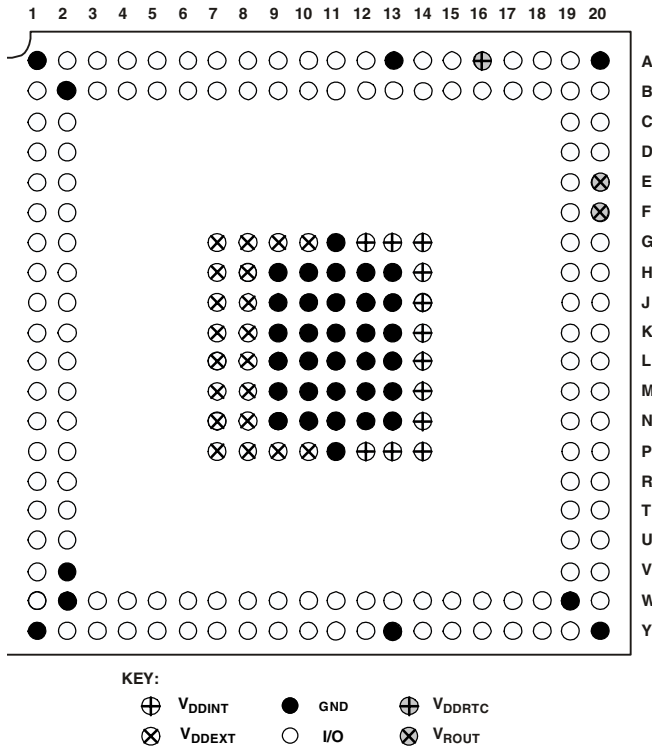
Figure 64. 208-Ball Mini-BGA Configuration (Top View)
