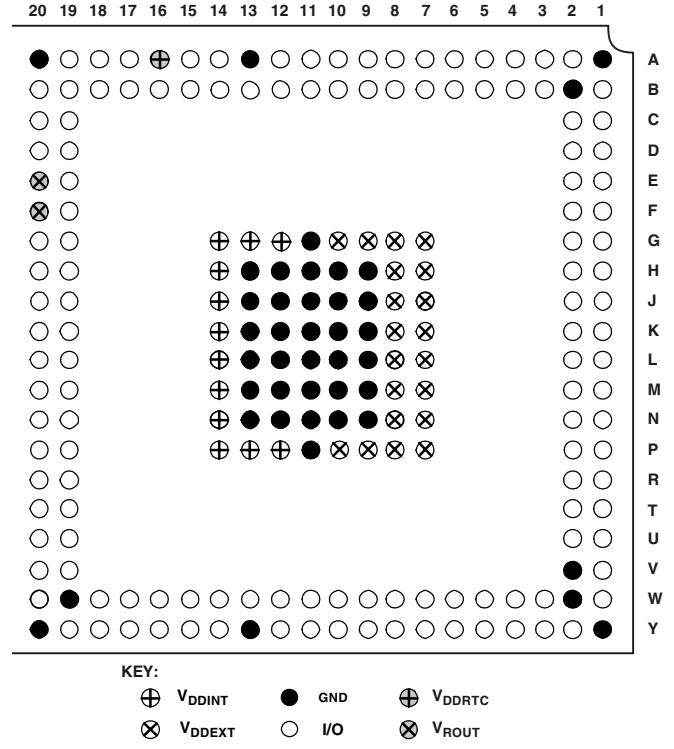
Figure 65. 208-Ball Mini-BGA Configuration (Bottom View)
