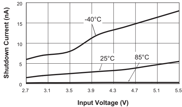
Shutdown Current vs. Input Voltage ( V_{EN/SET} = V_{ENA/ENB} = 0V )
