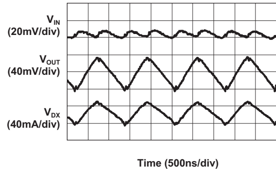
Backlight Operating Characteristic ( V_{IN} = 2.9V ; 2X Mode; 20mA/Channel Load; AC Coupled)
