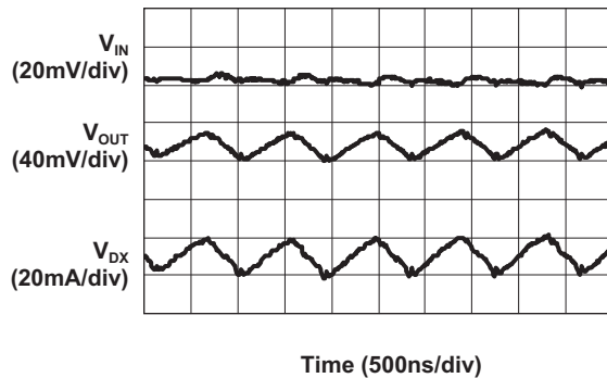
Backlight Operating Characteristic ( V_{IN} = 3.5V ; 1.5X Mode; 14mA/Channel Load; AC Coupled)
