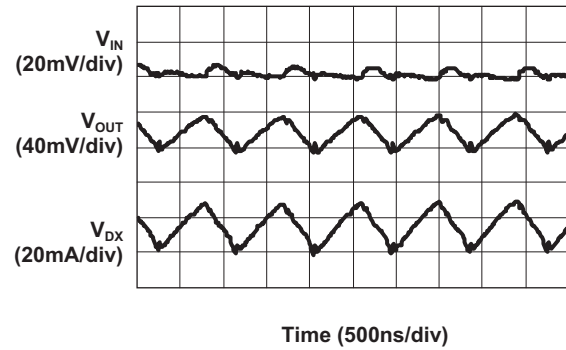
Backlight Operating Characteristic ( V_{IN} = 3.7V ; 1.5X Mode; 20mA/Channel Load; AC Coupled)
