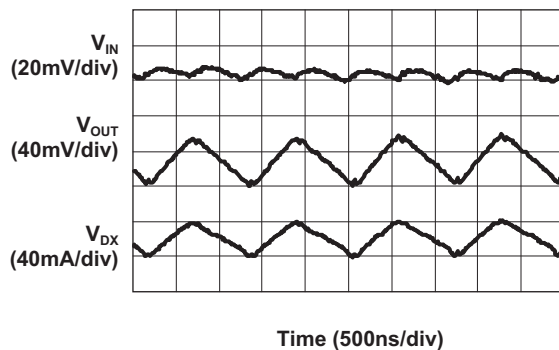
Backlight Operating Characteristic ( V_{IN} = 2.9V ; 2X Mode; 14mA/Channel Load; AC Coupled)
