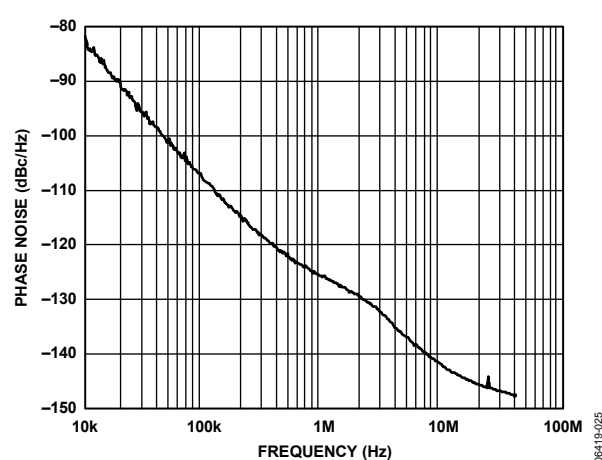
Figure 30. Internal VCO Phase Noise (Absolute) Direct to LVPECL @ 2550 MHz
