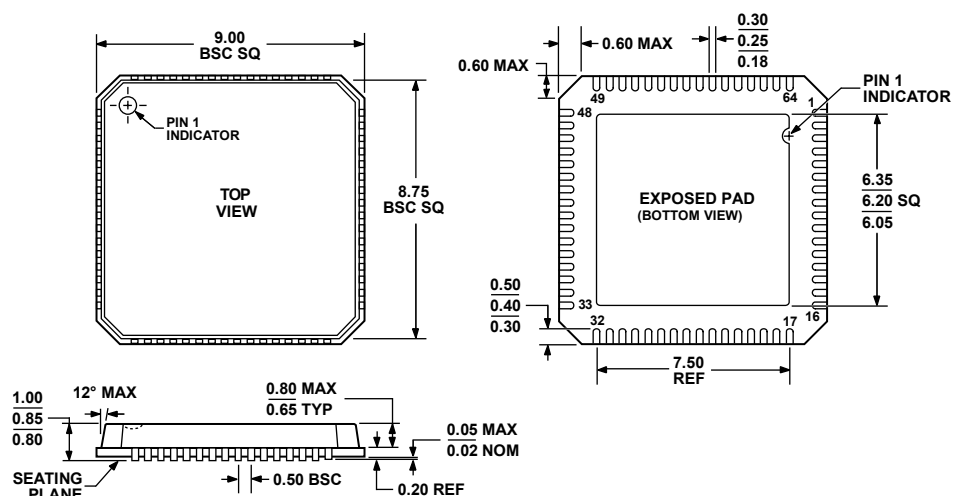
Figure 74. 64-Lead Lead Frame Chip Scale Package [LFCSP_VQ] 9 mm × 9 mm Body, Very Thin Quad CP-64-4
