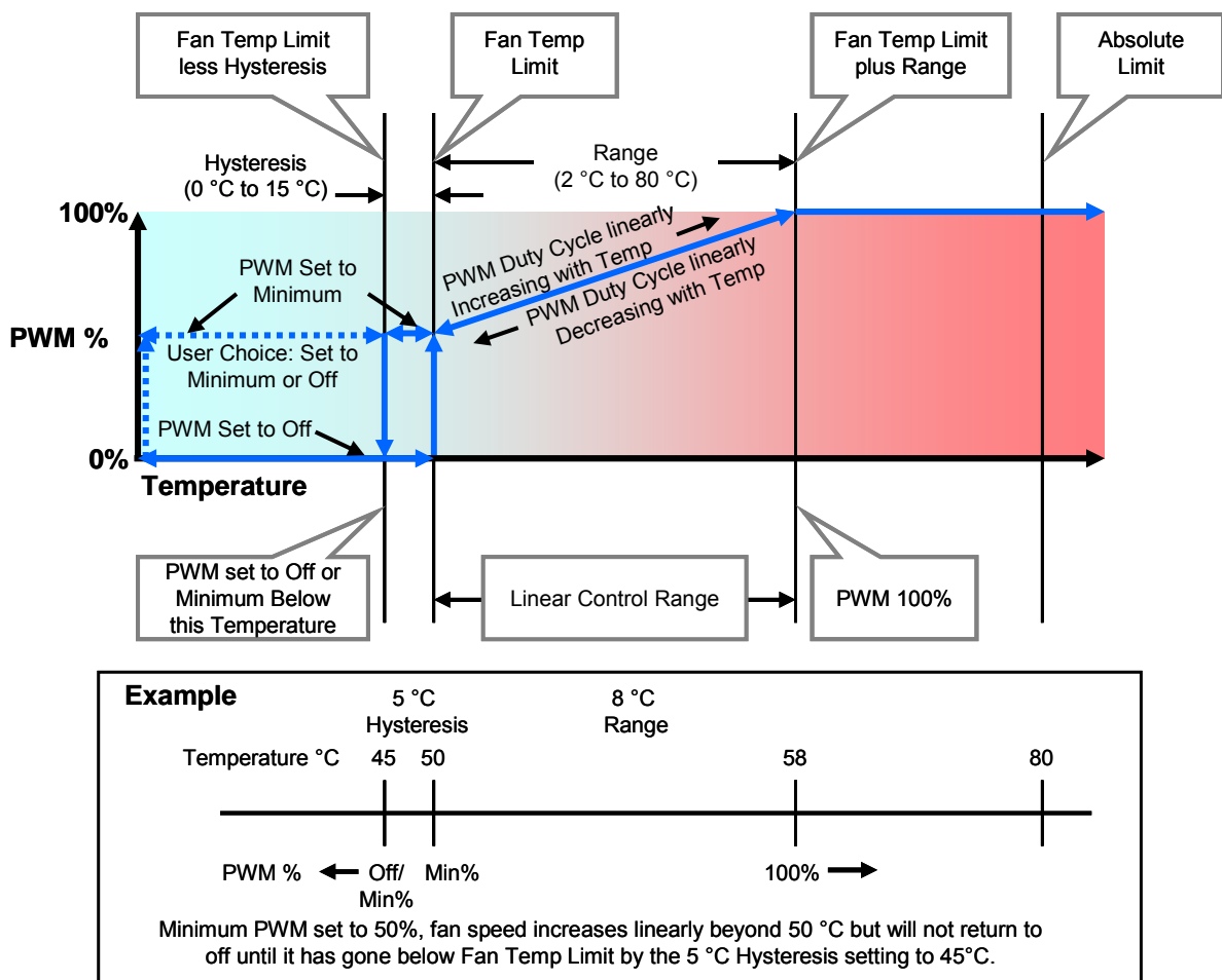
Figure 6 Automatic Fan Speed Control Example
