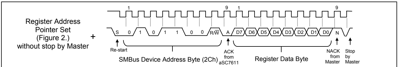
Figure 4 Register Read
