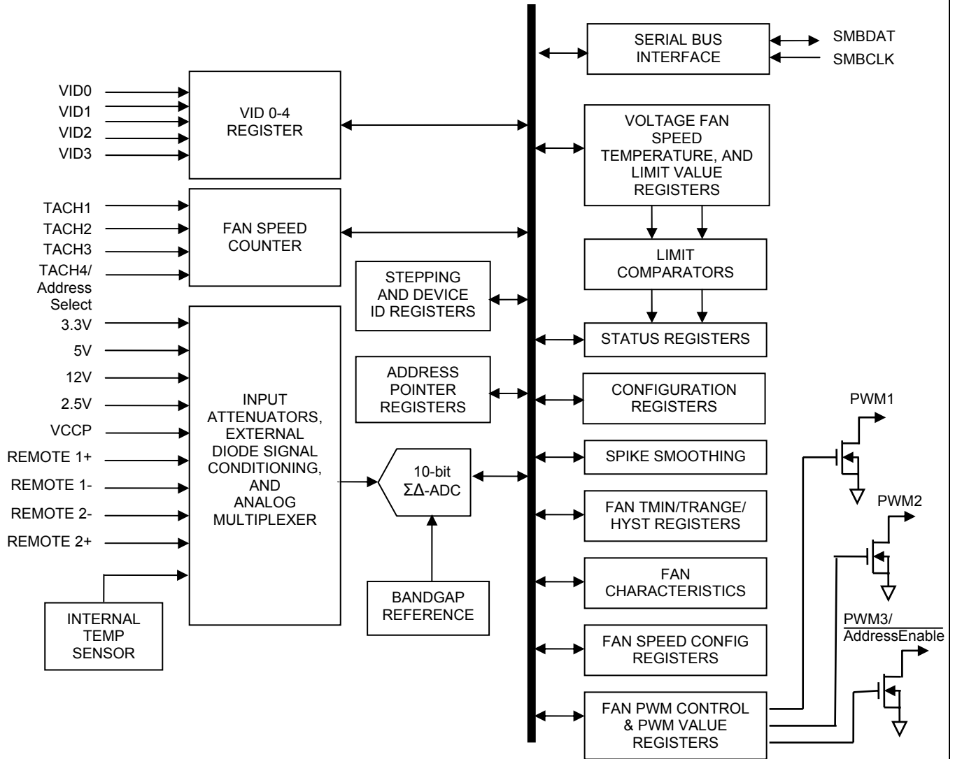
Figure 1 Block Diagram
