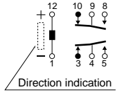
Schematic (Top view) Single side stable (Deenergized condition) 1 coil latching (Reset condition)
