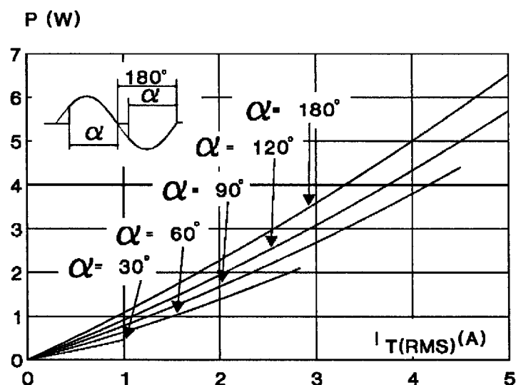
Fig. 1 :Maximum RMS power dissipation versus RMS on-state current (F = 60Hz). (Curves are cut off by (di/dt) c limitation)
