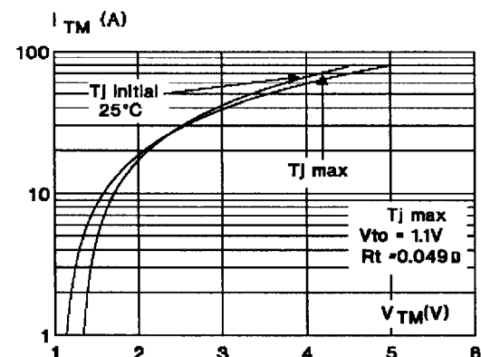
Fig. 5 :On-state characteristics (maximum values).
