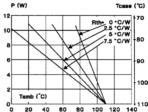
Fig. 3 :Correlation between maximum mean power dissipation and maximum allowable temperatures ( T_{amb} and T_{case} ) for different thermal resistances heatsink + contact (AVS10CBI).
