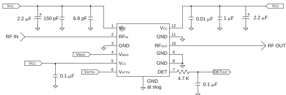
Figure 16: Application Circuit
