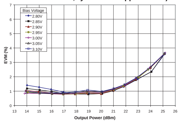
Figure 9: Effects of Bias Voltage ( V_{BIAS} ) on EVM ( T_C = +25^\circ\text{C} , V_{CC} = +6.0\text{ V} , f = 3.5\text{ GHz} , 54 Mbps OFDM Modulation, system EVM Approx. 0.8 %)
