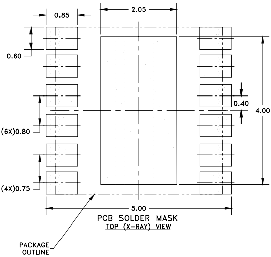
Figure 17: Land Pattern
