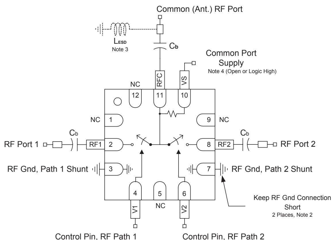
Figure 9: Application Schematic
