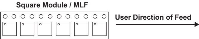
Figure 12: Tape & Reel Package Orientation
