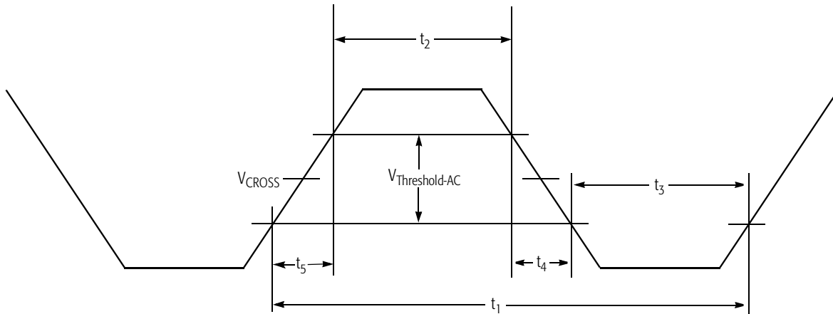
Figure 8. SYSCLK Waveform
