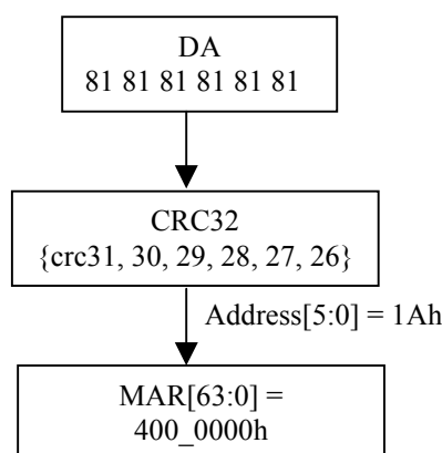
Figure 5: Multicast Filter Example
