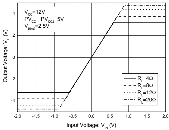
Figure 7. Driver I/O Characteristics (Sled)
