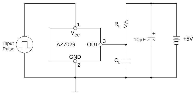
Figure 5. Test Circuit 2
