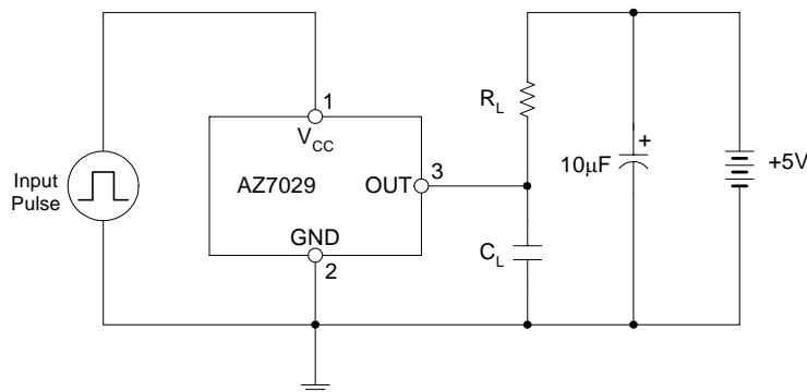
Figure 5. Test Circuit 2
