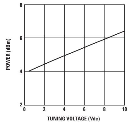
Figure 3. Power Output.
