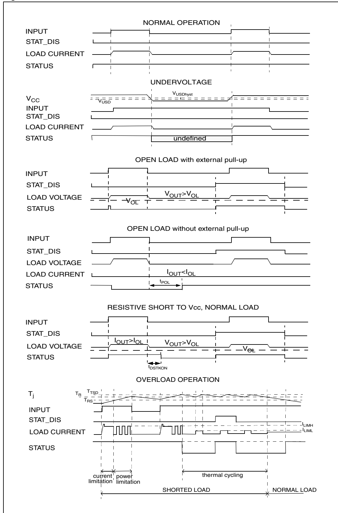
Figure 7. Waveforms
