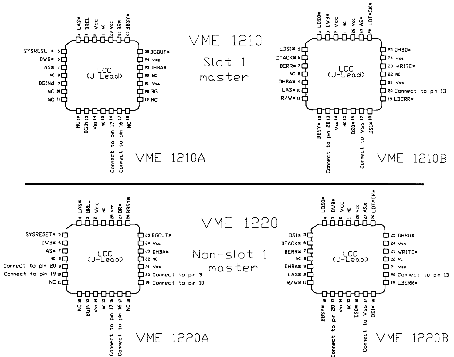
Figure 2. Pinout of VME 1210/1220 (LCCs)
