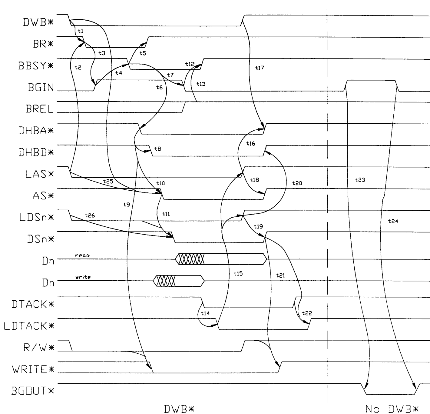
Figure 5. Timing Diagram
