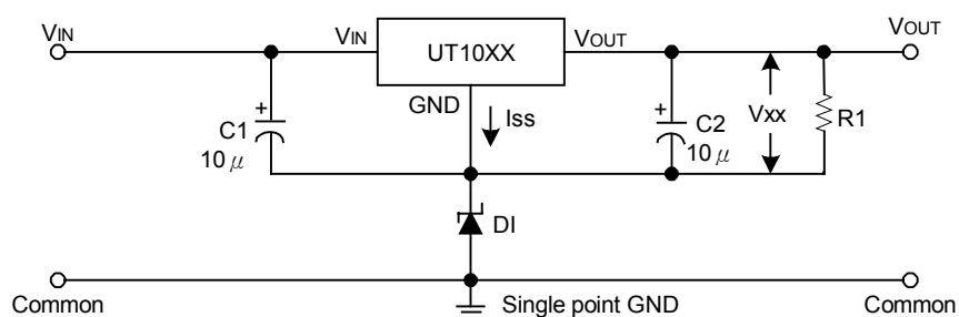
Circuit for increasing output voltage
