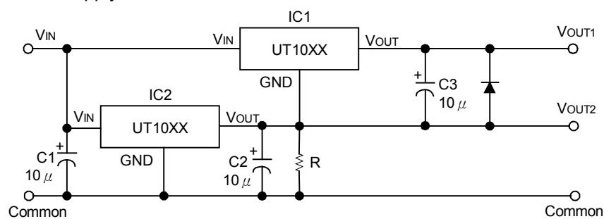
Dual supply
