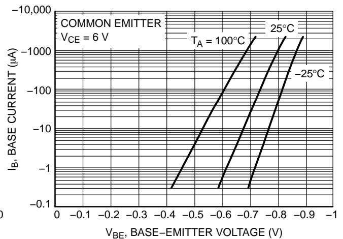
Figure 6. Base-Emitter Voltage
