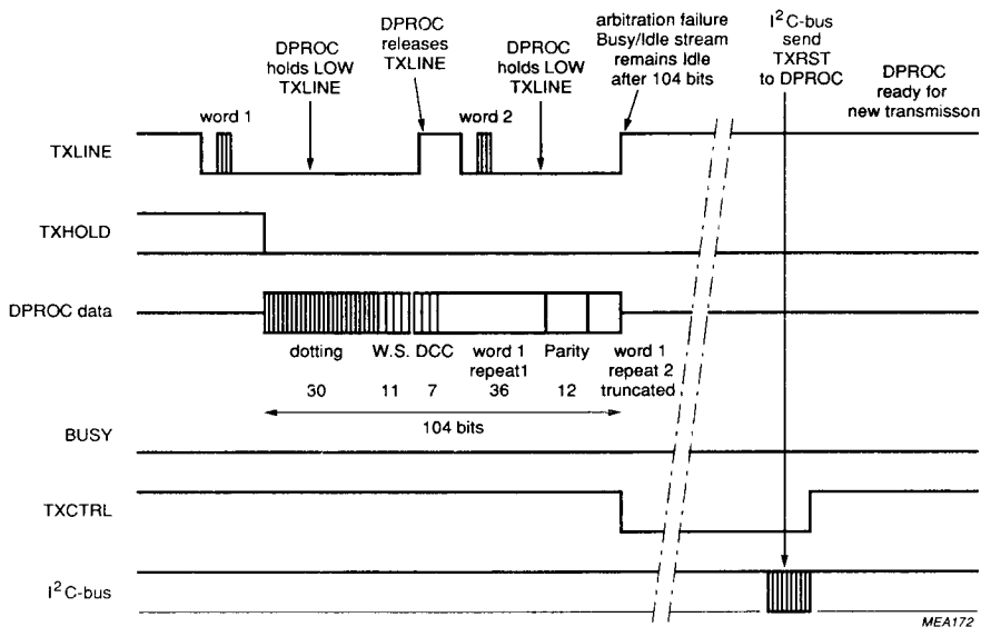
Fig.18 DPROC data transmission timing/microcontroller interface during arbitration failure.
