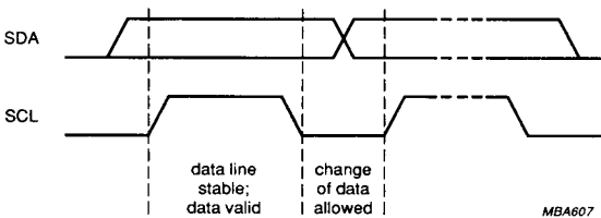
Fig.8 Bit transfer.
