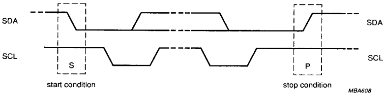
Fig.9 Definition of start and stop conditions.
