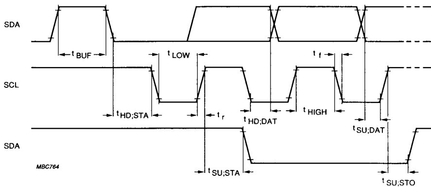
Fig.12 Timing.
