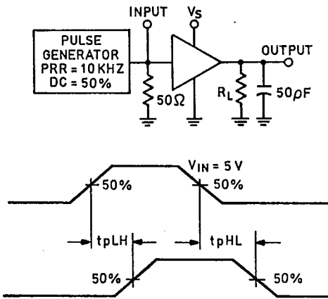
Dwg. No. A-13,26A
