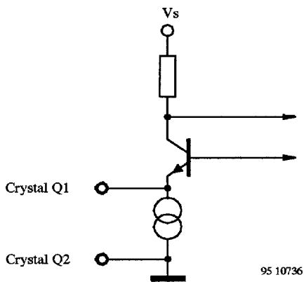
Figure 8. Reference oscillator
