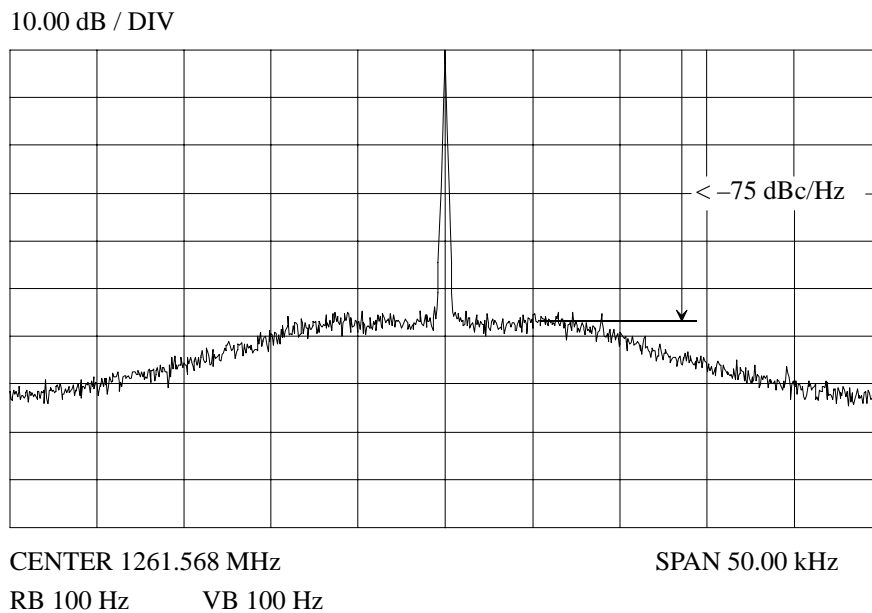
Figure 7. Phase noise
