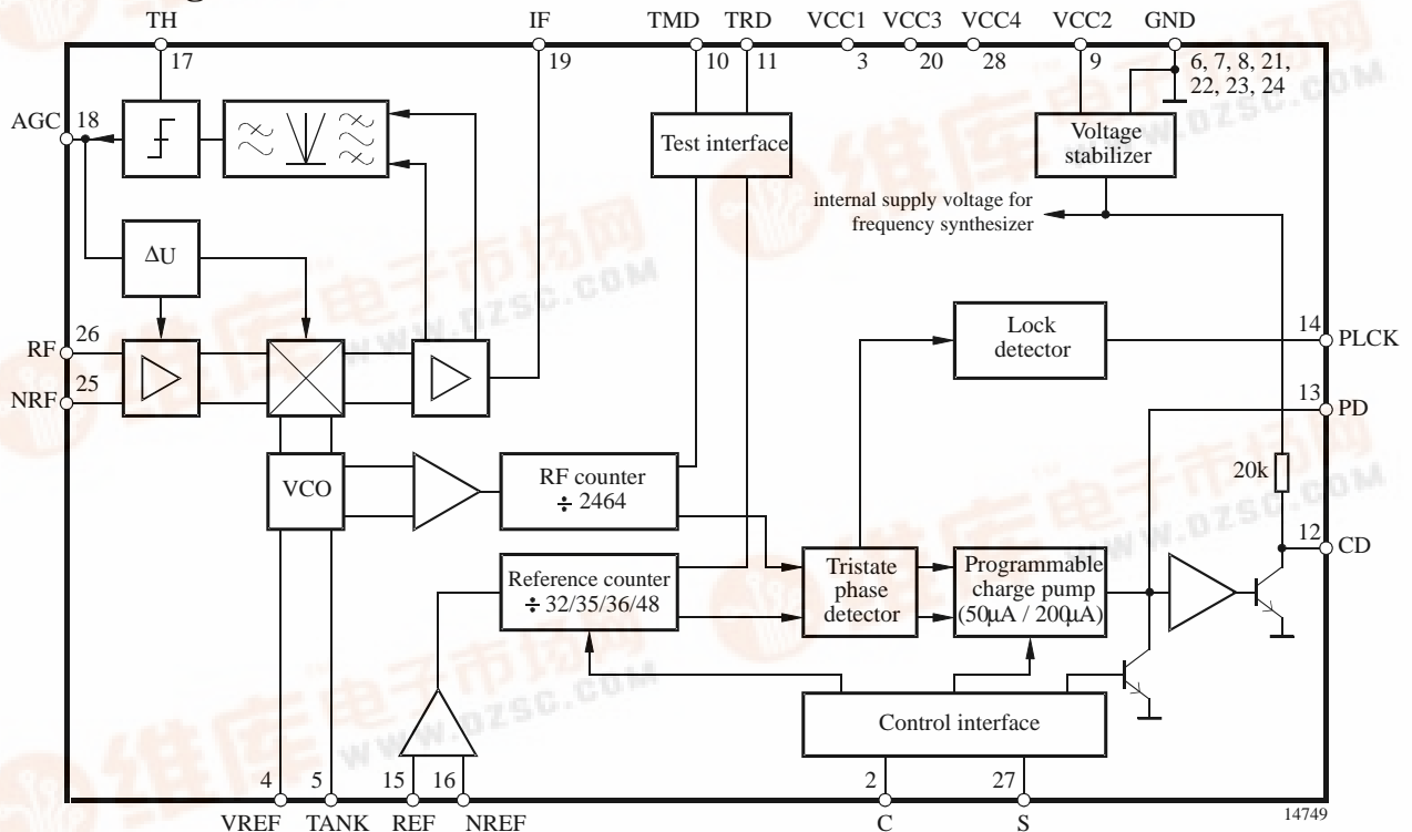
Figure 1. Block diagram
