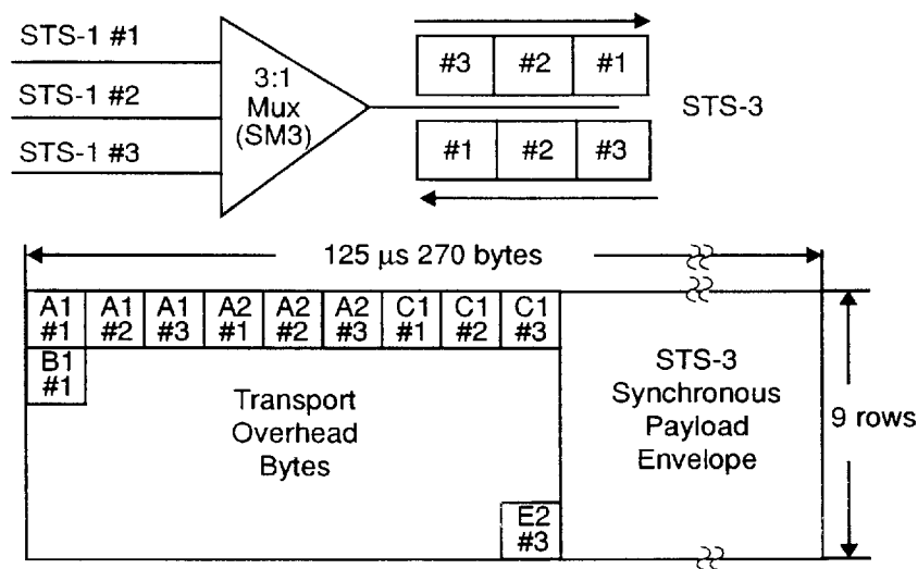
Figure 2. STS-3 Format
