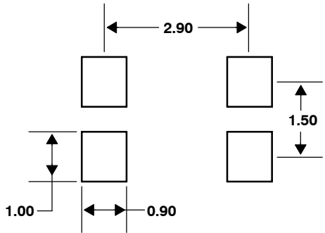
Figure 15. Suggested T Package PCB Layout
