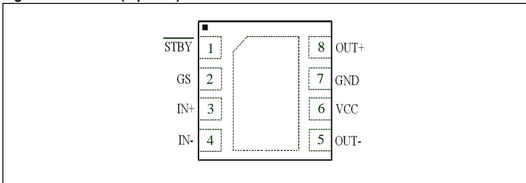
Figure 52. Pinout (top view)
