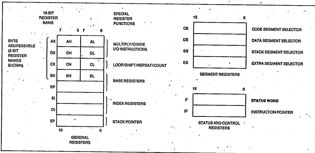
Figure 3a. 80C186 Register Set
