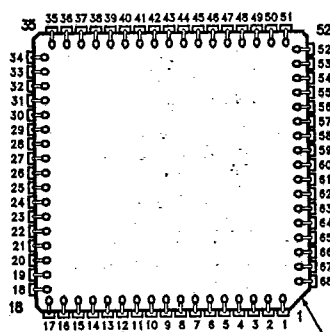
Figure 2. 80C186 Pinout Diagrams
