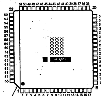
Figure 2. 80C186 Pinout Diagrams
