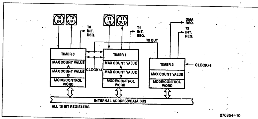
Figure 19. Timer Block Diagram
