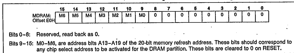
Figure 40. Memory Partition Register
