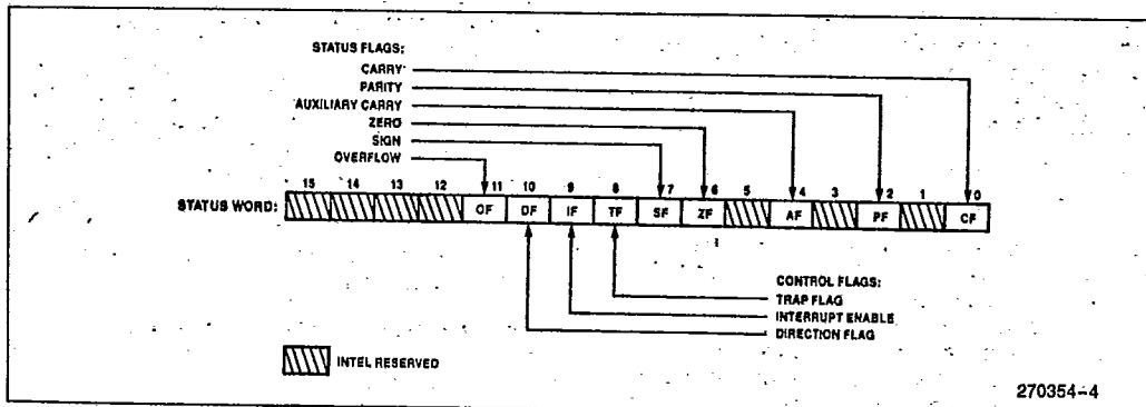
Figure 3b. Status Word Format 24-67
