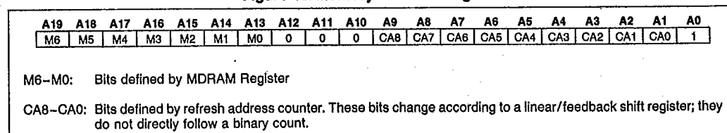
Figure 41. Addresses Generated by RCU
