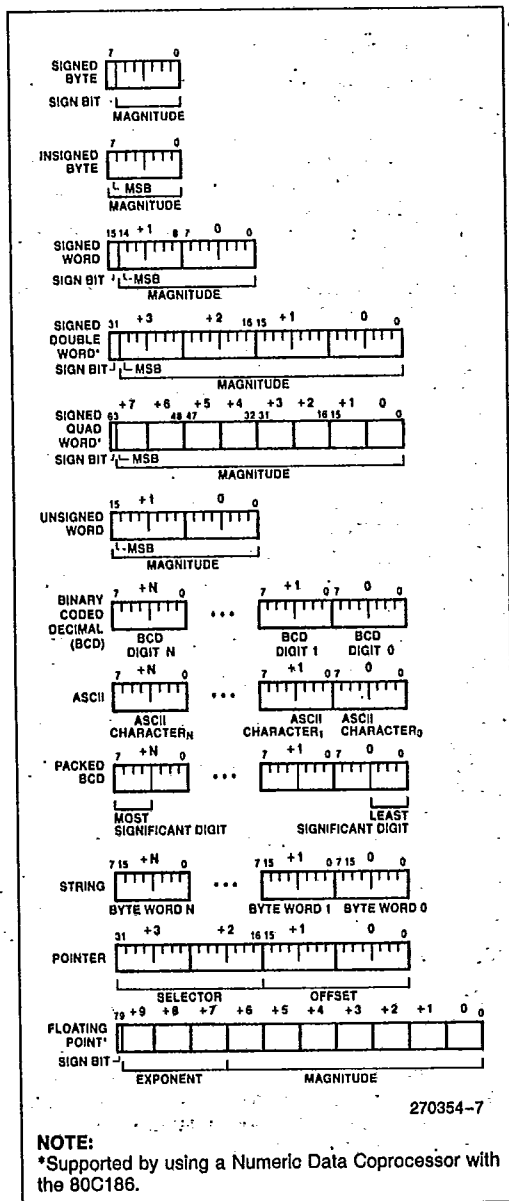
Figure 7. 80C186 Supported Data Types
