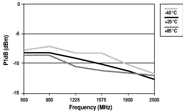
P1dB vs. Frequency vs. Temperature
