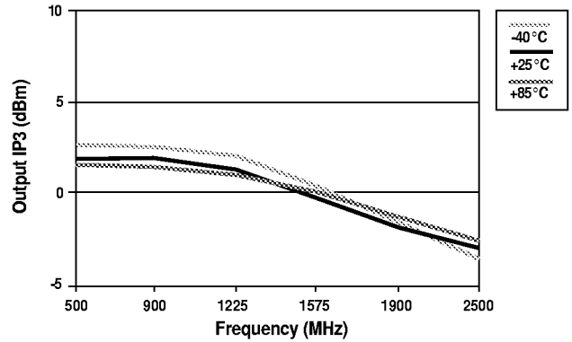
IP3 vs. Frequency vs. Temperature
