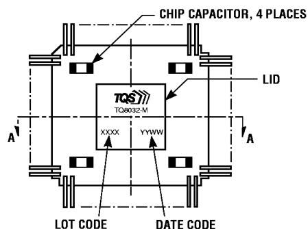
Figure 7. Mechanical Dimensions
