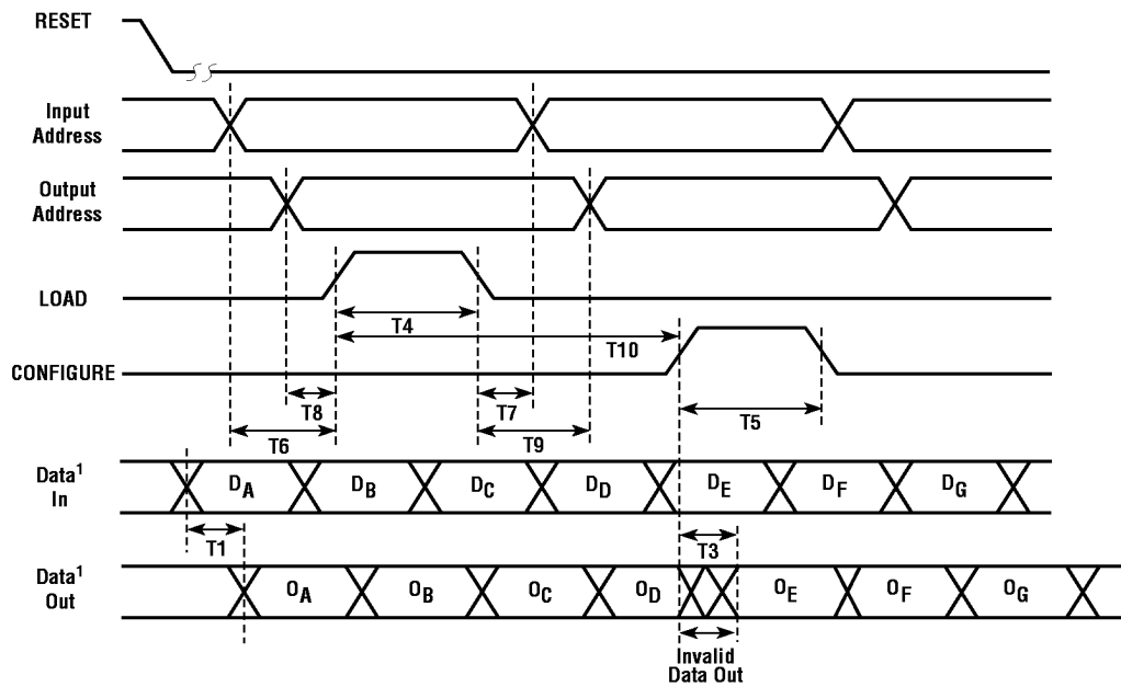
Figure 3. Timing Diagram – Switch Configuration
