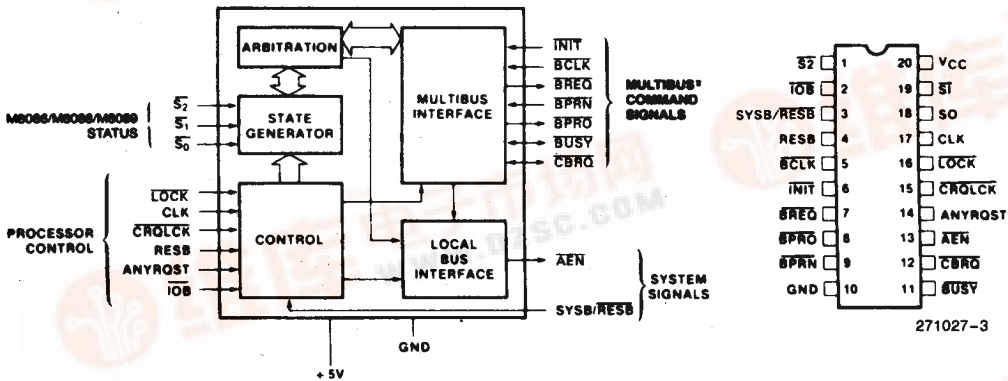
Figure 1. Block Diagram
