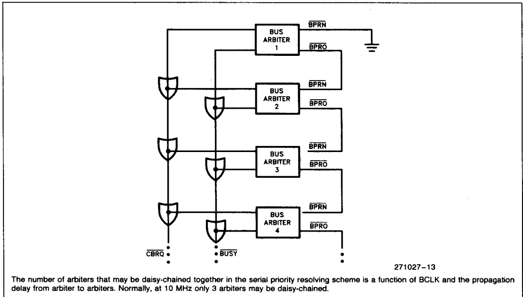
Figure 6. Serial Priority Resolving
