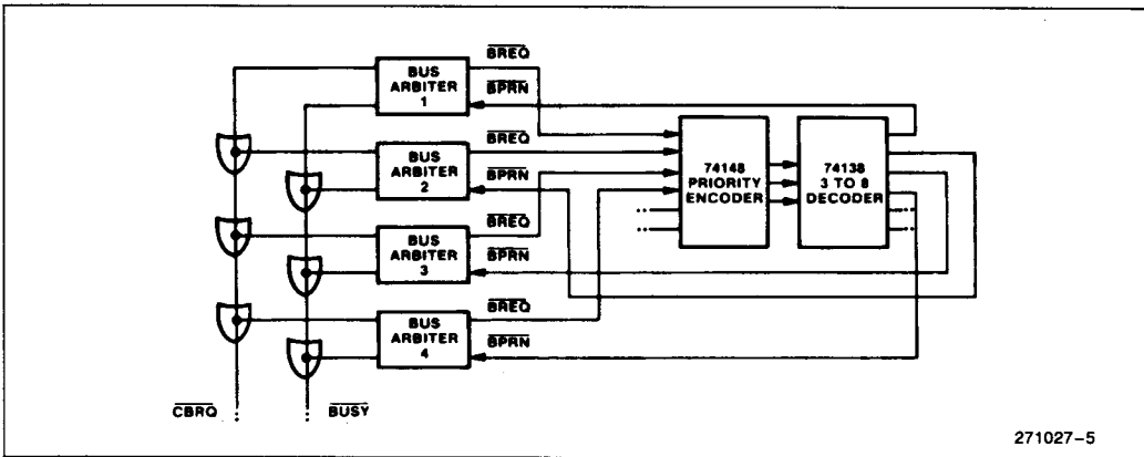
Figure 4. Parallel Priority Resolving Technique
