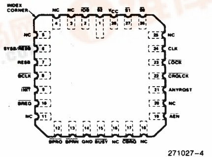
Figure 3. M8289 Pin Diagram
