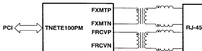
Figure 2. Schematic for 10 Base-T Network Interface Using TNETE100PM
