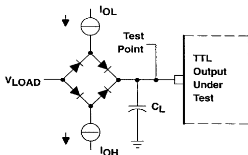
(a) TTL OUTPUT TEST LOAD
