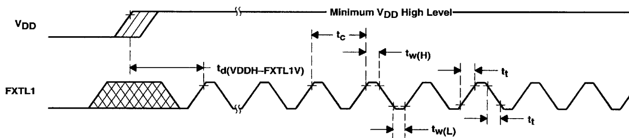
Figure 10. Crystal-Oscillator Timing
