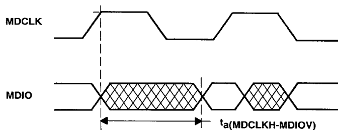
Figure 6. Management Data I/O Timing (Sourced by PHY)
