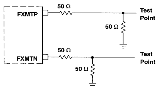
(e) FXMTP AND FXMTN TEST LOAD (dc TESTING)
