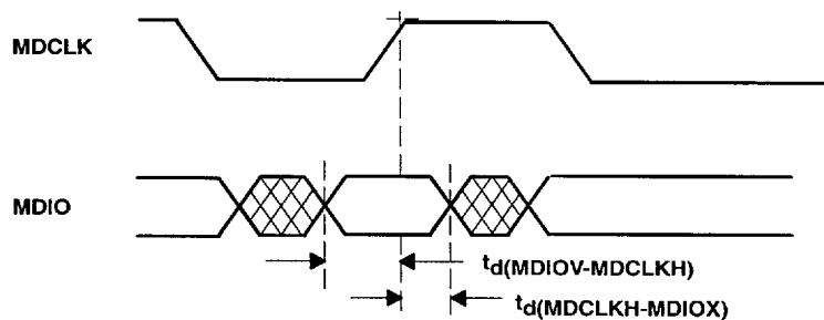
Figure 7. Management Data I/O Timing (Sourced by TNETE100PM)
