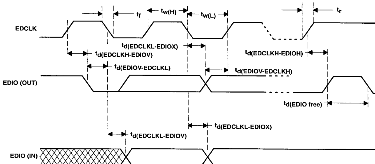
Figure 9. Configuration EEPROM Interface Timing
