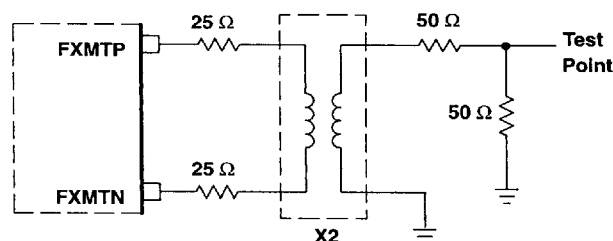
(d) FXMTP AND FXMTN TEST LOAD (ac TESTING) X2 – Fil – Mag 23Z128 (1:√2)
