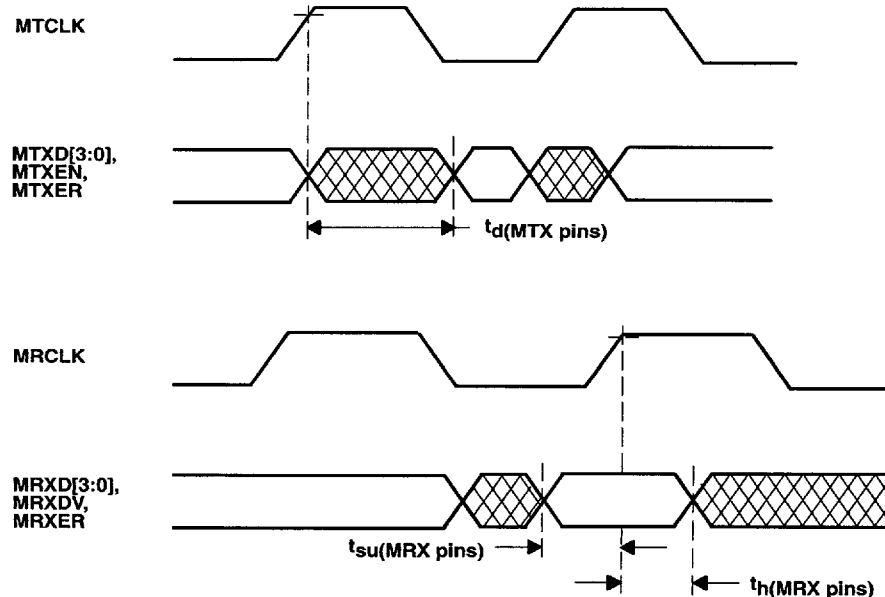
Figure 5. MII Transmit and Receive Timing
