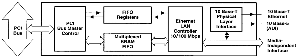
Figure 1. ThunderLAN Architecture
