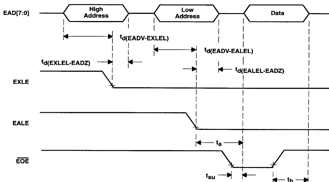
Figure 8. BIOS ROM and LED Interface Timing
