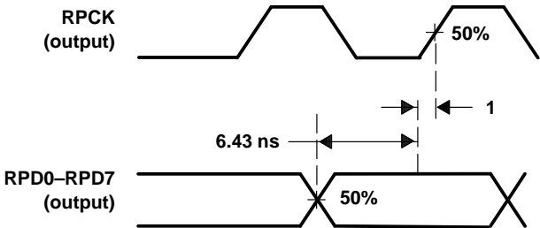
Figure 3. Receive Parallel Interface
