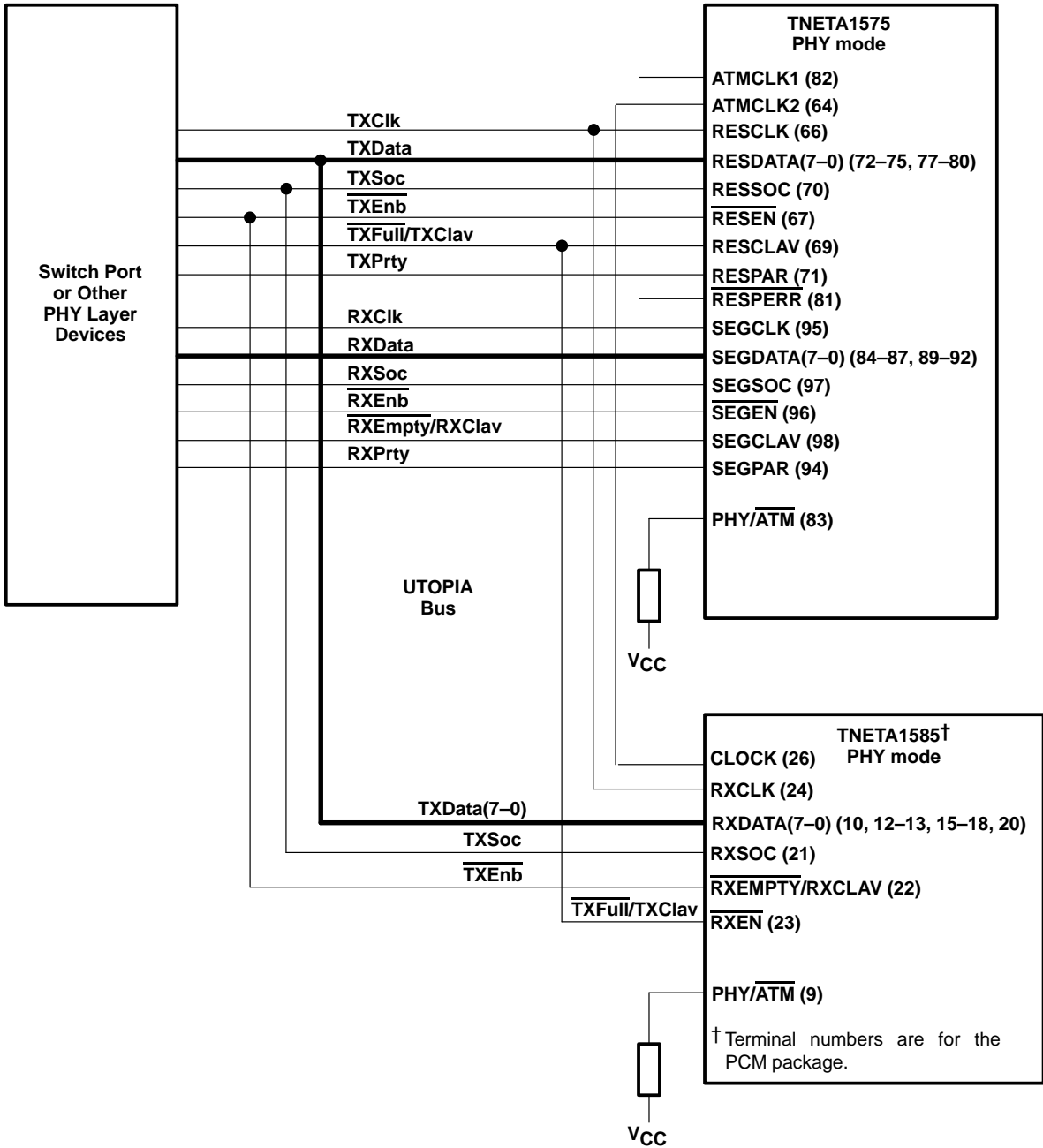
Figure 2. UTOPIA Bus Connections In PHY Mode
