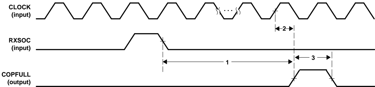
Figure 13. COPFULL Timing
