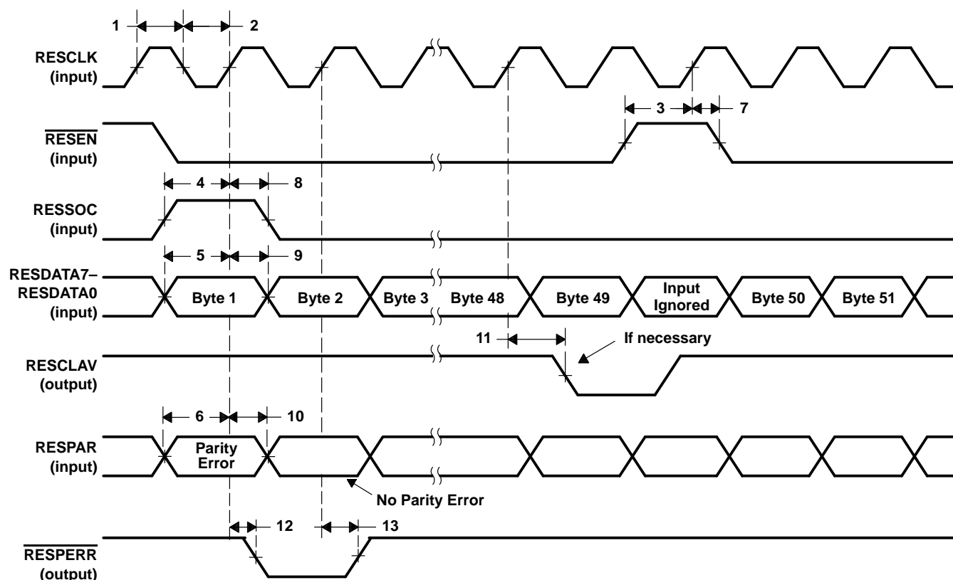
Figure 3. Reassembly-Cell Interface (PHY/ATM High)
