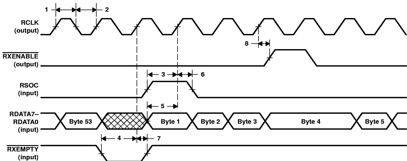
Figure 1. Receive-Cell Interface
