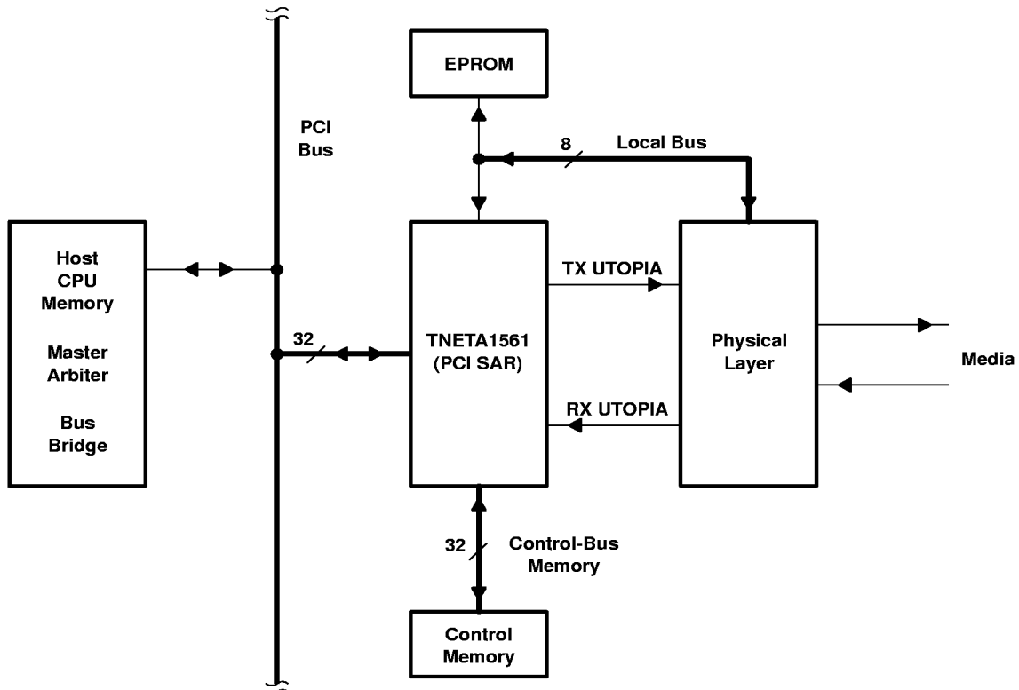
Figure 11. TNETA1561 Architecture
