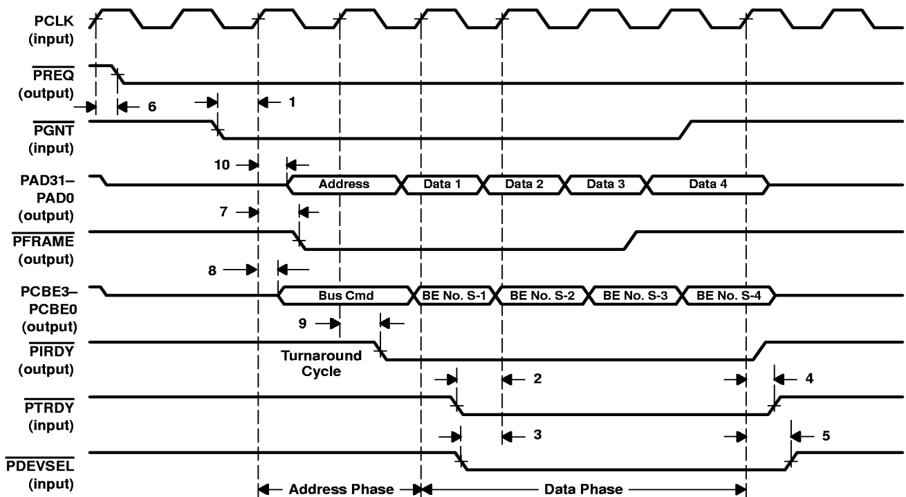
Figure 3. TNETA1561 Write Operation (PCI SAR as Master)
