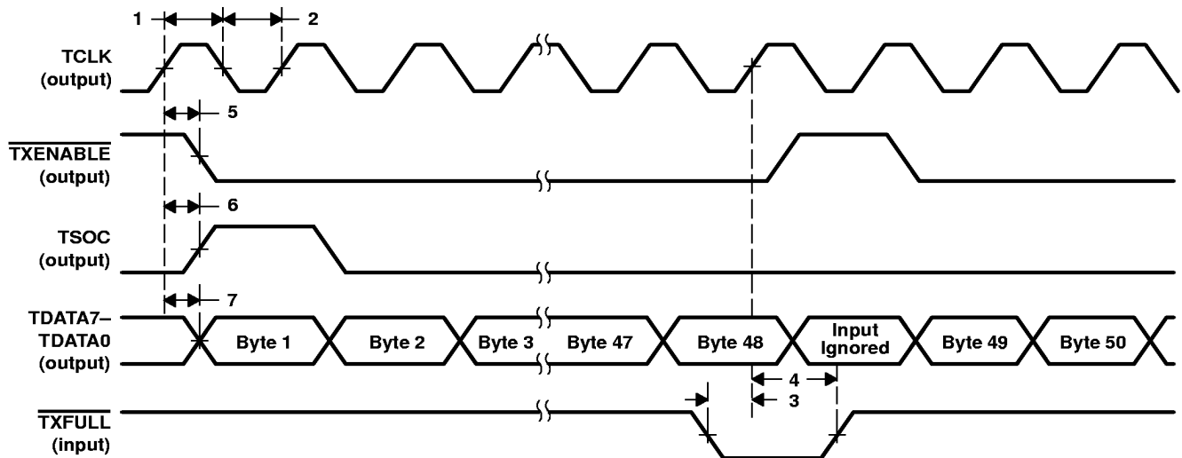
Figure 2. Transmit-Cell Interface
