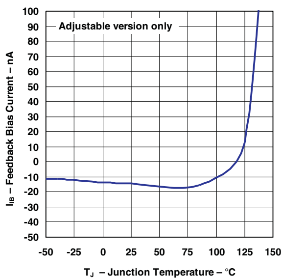
Figure 12. FEEDBACK Current
