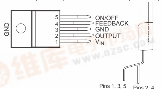
KV (TO-220 STAGGERED LEADS) PACKAGE (TOP VIEW)
