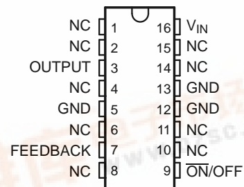
N (PDIP) PACKAGE (TOP VIEW)
