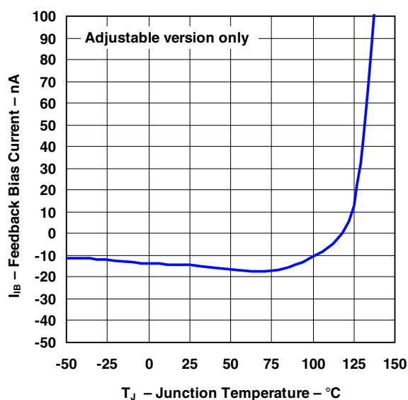
Figure 12. FEEDBACK Current
