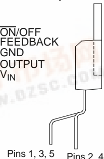
KV (TO-220 STAGGERED LEADS) PACKAGE (TOP VIEW)
